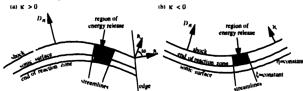
Figure 1. A snapshot showing diverging detonation (a), converging detonation (b), the intrinsic coordinates and the definition of the boundary-edge angle \omega . The speed of the wave is influenced by two factors, the convergence/divergence and the location of the sonic surface.
