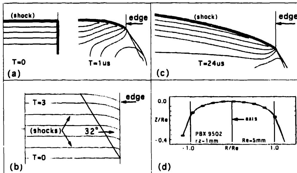
Figure 4. Response of a detonation reaction zone to a sudden loss of confinement. Insets (a), (b), (c) and (d) show the reaction-zone pressure contours, the evolving shock front shape, late time pressure contours and an experimentally measured shock-front shape, respectively.
