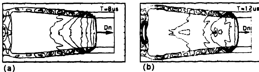
Figure 3. Mesa calculation of the detonation cylinder test. The detonation wave is moving to the right. Inset (a) shows the results at t = 8 \mu\text{s} from the D_n = D_{c,j} model. (b) shows the D_n(\kappa) model at t = 12 \mu\text{s} .
